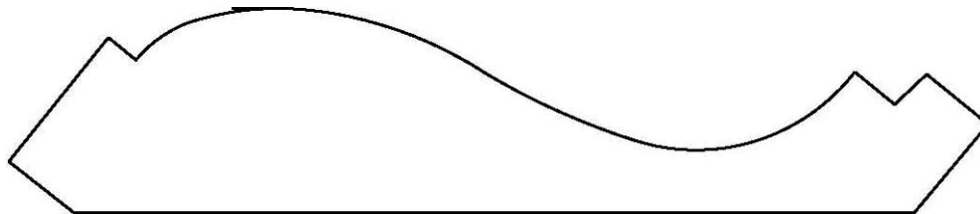
TAW07207 1-1/16" x 5-1/8"
