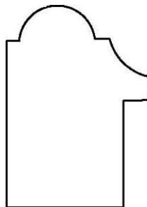
TAW07213 1-1/2" x 1-1/16" 3/16" x 3/4" Rab.
